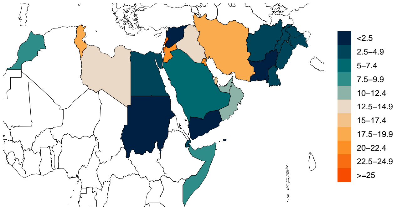
Figure 23. Forecasted percent infected with COVID-19 on June 01, 2021
