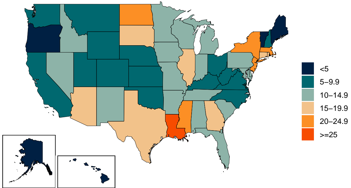
Figure 5. Percent of COVID-19 infections detected. This is estimated as the ratio of reported daily COVID-19 cases to estimated daily COVID-19 infections based on the SEIR disease transmission model.
