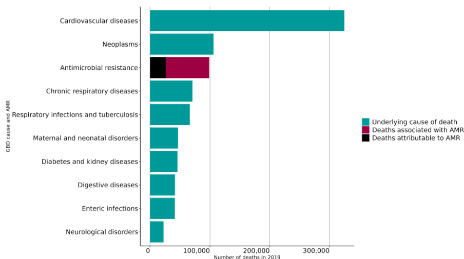
Figure 3. Placing AMR in context with other causes of death in 2019, Bangladesh
