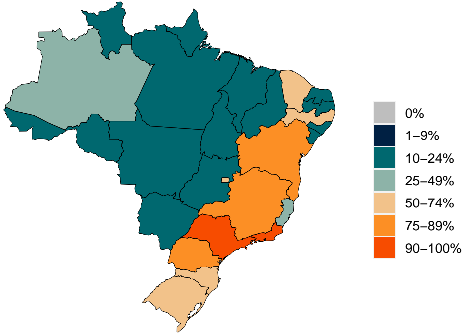
Figure 9.5 Estimated percent Omicron variant
