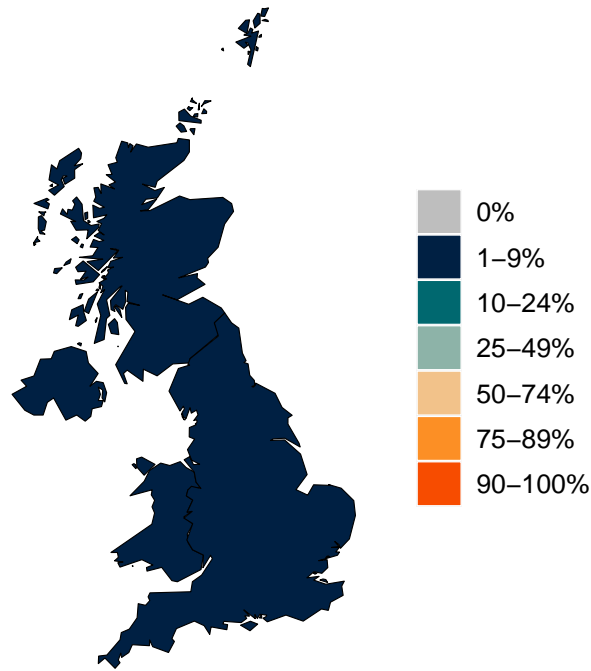
Figure 8.2: Estimated percent of new infections that are Beta variant
