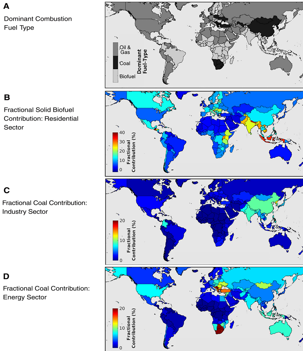
Figure 8. Fractional contributions from select combustion fuel types and sectors in 2017. (A) The combustion fuel type with the largest relative contribution to PM 2.5 mass and mortality in each country. (B–D) The fractional contributions to PM 2.5 mass and attributable mortality from solid biofuel combustion in the residential sector (B), coal combustion in the industry sector (C), and coal combustion in the energy sector (D). Note the color scale change between panels B and C–D.
