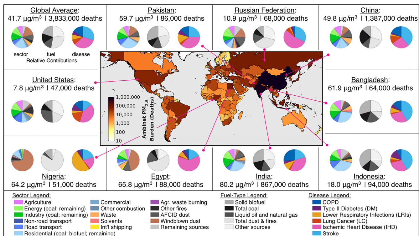
Figure 5. Ambient PM_{2.5} burden, population-weighted mean PM_{2.5} mass and fractional source sector, fuel, and disease contributions globally and for the nine countries with the largest burden. Map: National-level outdoor PM_{2.5} disease burden in 2017 (from 2019 GBD concentration–response function). Panels: Annual population-weighted mean PM_{2.5} exposure levels and attributable deaths (rounded to the nearest 1,000) for each country/region. Pie charts in each panel: (Left) fractional sectoral source contributions. “Other fires” include deforestation, boreal forest, peat, savannah, and temperate forest fires. Remaining sectoral sources include volcanic SO_2 , lightning NO_x , biogenic soil NO , and oceanic and biogenic emissions (Table 1). Energy and industry sectors show separate contributions from coal use (lighter green); the residential sector separates contributions from coal and solid biofuel (two light blue wedges). (Middle) fuel-type contributions. “Total dust & fires” is the sum of windblown dust and AFCID dust (anthropogenic fugitive, combustion, and industrial dust), agricultural waste burning, and other fires. Other sources are noncombustion or uncategorized combustion sources (waste incineration, agriculture, solvents, biogenic secondary organic aerosols, etc.). (Right) relative disease contributions.
