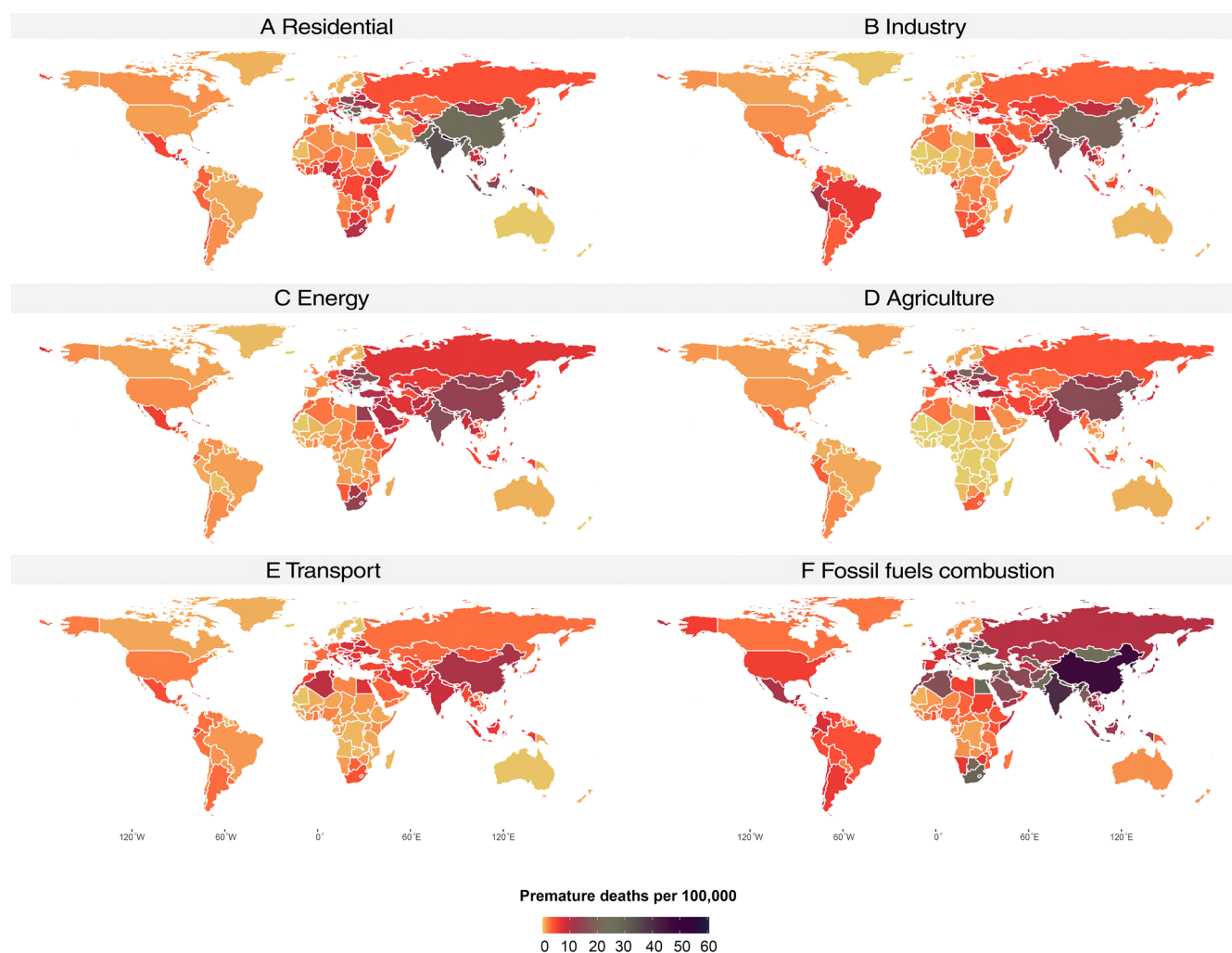
Figure 7. Premature deaths per 100,000 attributable to population-weighted mean ambient PM 2.5 mass from selected sectors in 2017. (A–E) The rate of deaths per 100,000 from residential, industry, energy, agriculture and transport (on road and nonroad) sectors in each country, respectively. (F) Deaths per 100,000 from all fossil fuel combustion (total coal plus liquid oil and natural gas) in each country.
