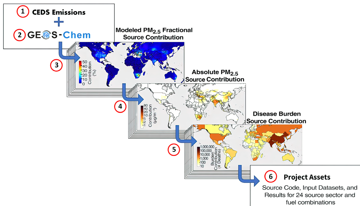
Figure 1. General schematic of the GBD MAPS global project methods. Each step is indicated by a number and is described in the main text. As an illustrative example, the modeled fractional, absolute, and PM 2.5 disease burden contributions from coal use in the energy sector are shown in Steps 3–5. These steps are repeated for each of the 24 individual source sector and fuel categories (Table 1). (Adapted from Hoesly et al. 2018; CC Attribution 4.0 License.)
