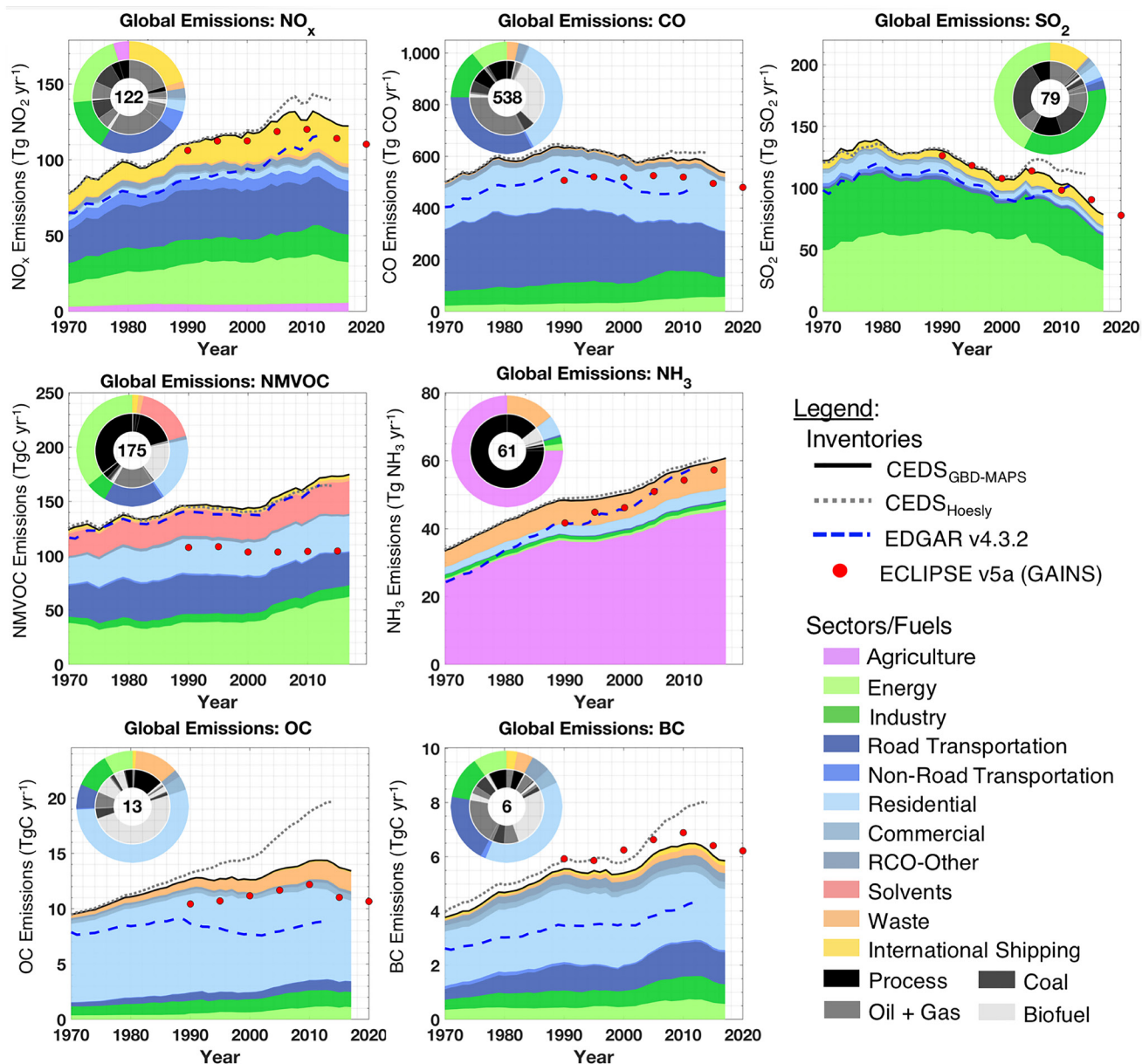
Figure 2. Time series of global annual emissions of NO x (as NO 2 ), CO, SO 2 , NMVOCs, NH 3 , BC, and OC for all sectors and fuel types. Solid black lines are the CEDS GBD-MAPS inventory, with fractional sector contributions indicated by colors. Dashed gray lines are the original CEDS Hoesly inventory. Dashed blue lines are the EDGAR v4.3.2 global inventory. Red dots are ECLIPSE v5a baseline “current legislation” emissions with data in 2015 and 2020 from GAINS CLE projections. All inventories include international shipping but exclude aircraft emissions. Pie chart inserts show fractional contributions of emission sectors to total 2017 emissions (outer) and fuel type contributions to each sector (inner). Emission totals for 2017 (units: TgC yr -1 for NMVOCs, OC, and BC) are given inside each pie chart.
