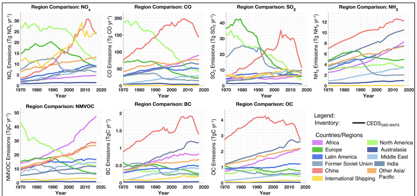
Figure 4. Time series of global annual \text{CEDS}_{\text{GBD-MAPS}} emissions of \text{NO}_x , \text{CO} , \text{SO}_2 , \text{NH}_3 , NMVOCs, BC, and OC for all sectors and fuel types (excluding aircraft emissions), split into ten countries/regions.
