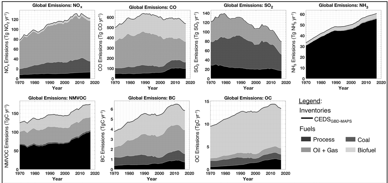
Figure 3. Time series of global annual emissions of \text{NO}_x , \text{CO} , \text{SO}_2 , \text{NH}_3 , NMVOCs, BC, and OC for all sectors, colored by fuel group.
