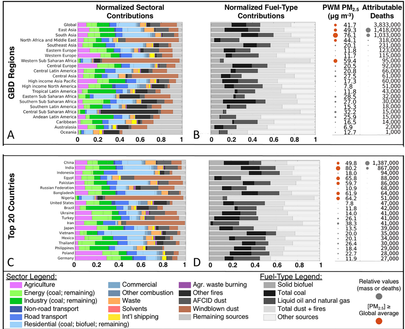
Figure 6. Relative source and fuel-type contributions to population-weighted mean ambient PM_{2.5} mass and attributable deaths. (A and C): Normalized sectoral source contributions for the global average and 21 world regions (A) and the 20 countries with the most attributable PM_{2.5} deaths (C), sorted by decreasing number of outdoor PM_{2.5} -associated deaths in 2017 (2019 GBD concentration–response functions, rounded to the nearest 1,000). (B and D): Normalized contributions from the combustion of three fuel types and remaining PM_{2.5} sources. Sector categories are the same as Figure 5. To the right of B and D are annual average population-weighted mean PM_{2.5} concentrations and associated attributable deaths for each region/country, with relative amounts illustrated by relative dot sizes. Concentrations above or equal to the global average are colored red.
